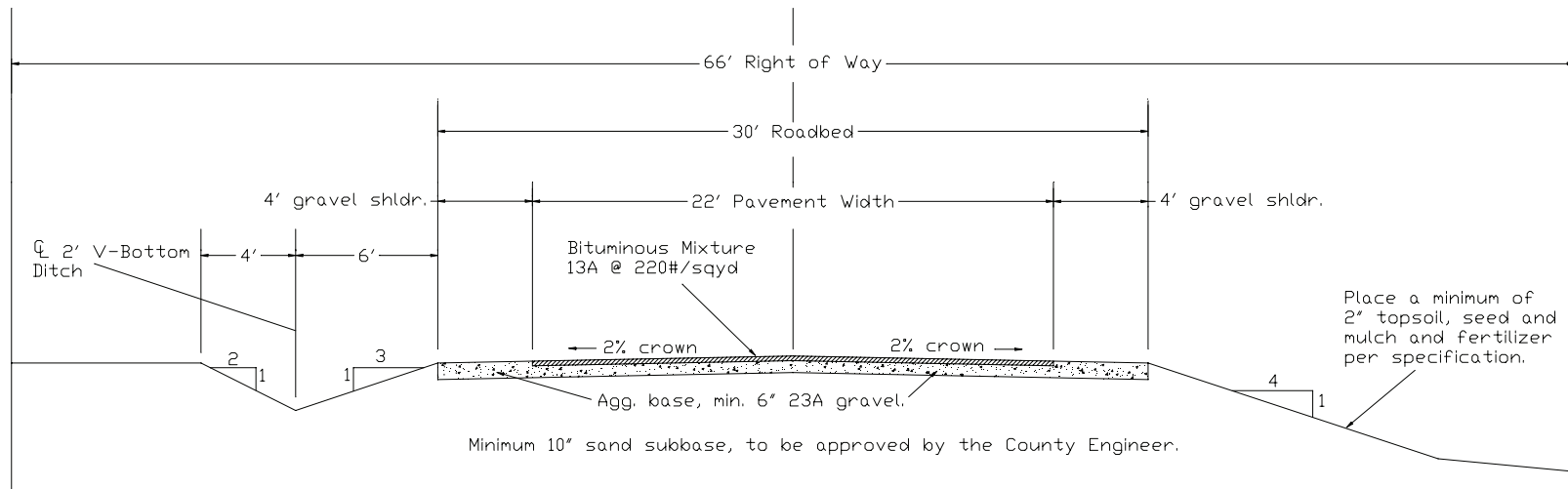
TYPICAL CROSS SECTION (WELL DRAINED SOIL)
